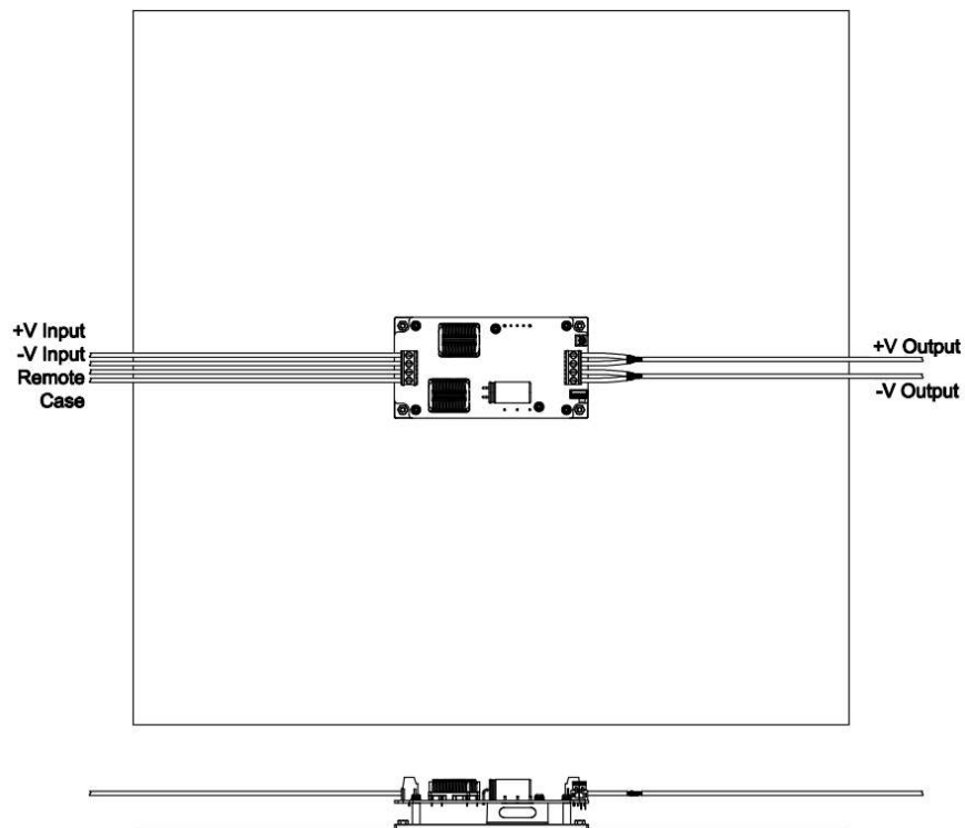
Figures 2 CQB100W-110SXX-CMFC with Heat Sink Aluminum Plate (17x17x0.04 inch)
