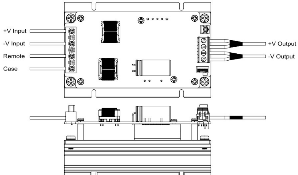
Figures 3 CQB100W-110SXX-CMFC with Heat Sink CMLH01
