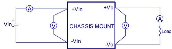
CQB100W-110SXX-CMFC(D) Series Test Setup
