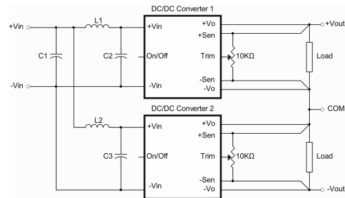
Simple ±Output Operation Connect Circuit
