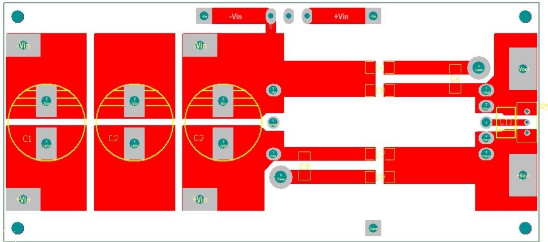
Figure3 PCB Layout Top View
