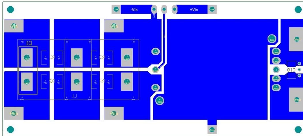
Figure4 PCB Layout Bottom View
