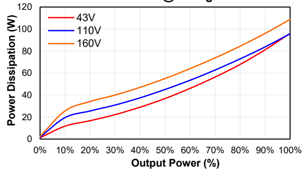
CFB600W-110S12 Pd Vs Po @25 Deg. C
