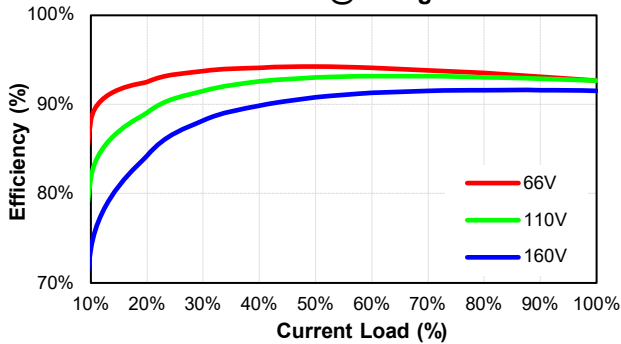
CHB150-110S05 Eff Vs Io @25 Deg. C
