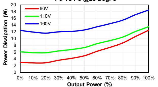
CHB150-110S24 Pd Vs Po @25 Deg. C
