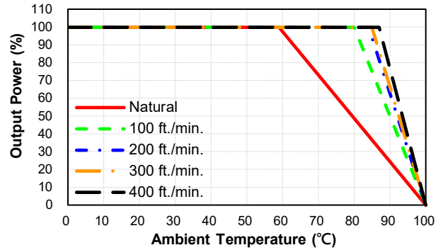
CHB150-110S24 Derating Curve with Heatsink HBT254 (Vin=110V)
