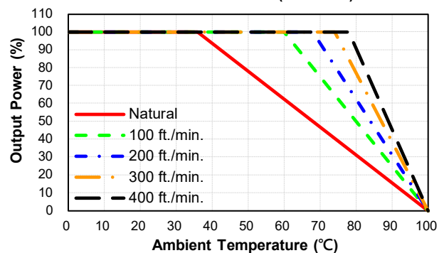
CHB150-110S24 Derating Curve with Heatsink HBT127 (Vin=110V)
