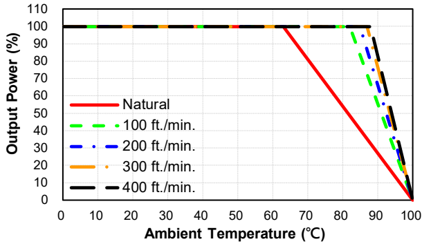
CHB150-110S05/12 Derating Curve with Heatsink HBT254 (Vin=110V)
