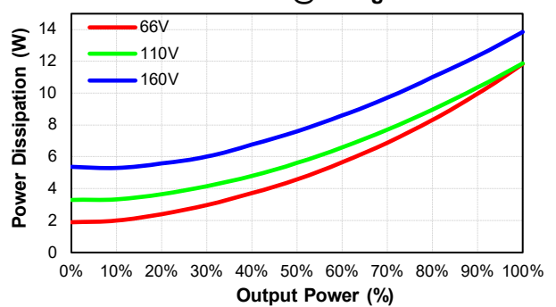
CHB150-110S05 Pd Vs Po @25 Deg. C
