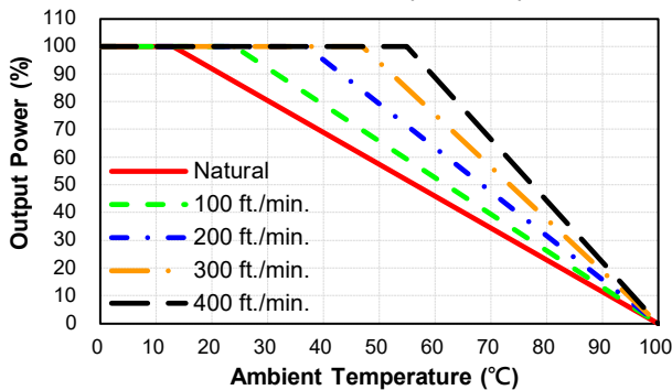
CHB150-110S05/12 Derating Curve without Heatsink (Vin=110V)
