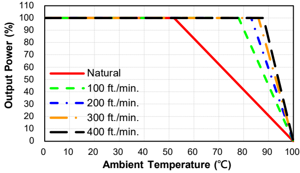
CHB150-110S05/12 Derating Curve with Heatsink HBL210 (Vin=110V)
