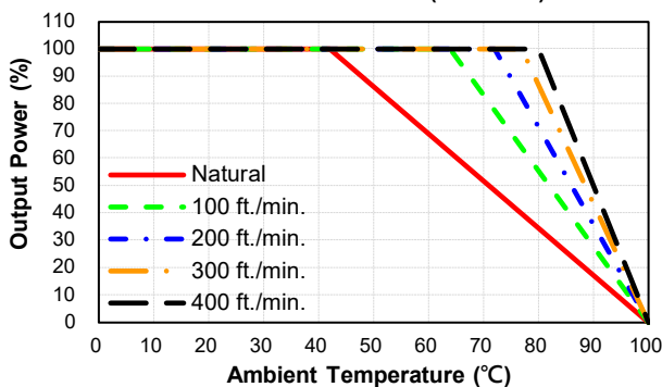
CHB150-110S05/12 Derating Curve with Heatsink HBT127 (Vin=110V)
