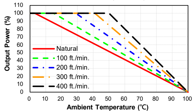
CHB150-110S24 Derating Curve without Heatsink (Vin=110V)
