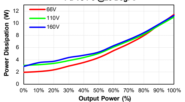
CHB150-110S12 Pd Vs Po @25 Deg. C
