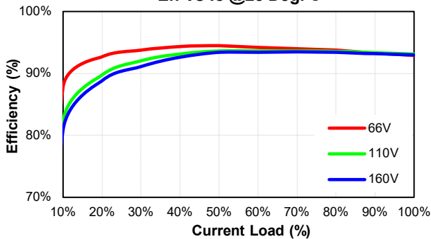
CHB150-110S12 Eff Vs Io @25 Deg. C
