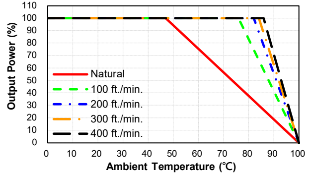
CHB150-110S24 Derating Curve with Heatsink HBL210 (Vin=110V)
