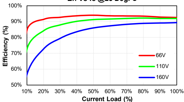
CHB150-110S24 Eff Vs Io @25 Deg. C
