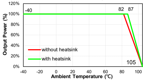
EC2SBW-XXS15H Derating Curve (Vin=Nominal)
