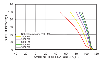
VTW150-4805S Derating Curve with 0.45" Height Heat Sink (See Thermal Conditions)
