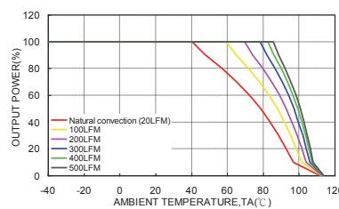
VTW150-4805S Derating Curve with 0.24" Height Heat Sink (See Thermal Conditions)
