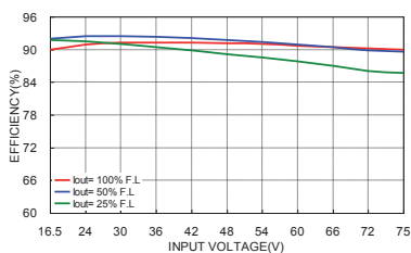
VTW150-4805S Efficiency vs. Input Voltage
