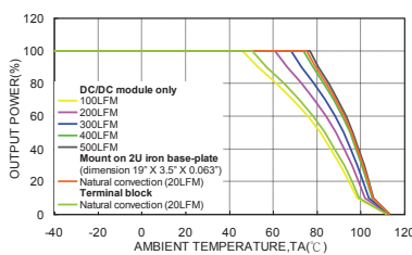
VTW150-4805S Derating Curve (See Thermal Conditions)
