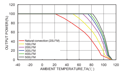
VTW200-4805S Derating Curve with 0.45" Height Heat Sink (See Thermal Conditions)
