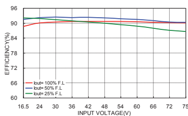
VTW200-4805S Efficiency vs. Input Voltage
