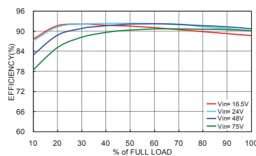
VTW200-4805S Efficiency vs. Output Voltage
