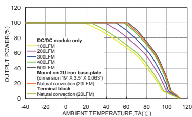
VTW200-4805S Derating Curve (See Thermal Conditions)
