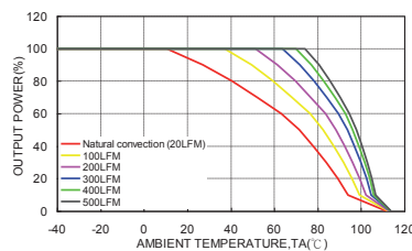
VTW200-4805S Derating Curve with 0.24" Height Heat Sink (See Thermal Conditions)
