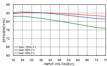
VTW75-4805SEfficiency vs. Input Voltage
