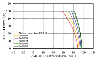
VTW75-4805S Derating Curve with 0.24" Height Heat Sink (See Thermal Conditions)
