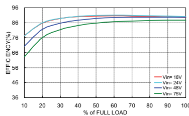
VTW75-4805SEfficiency vs. Output Voltage
