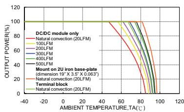
VTW75-4805S Derating Curve (See Thermal Conditions)
