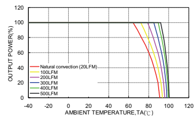
VTW75-4805S Derating Curve with 0.45" Height Heat Sink (See Thermal Conditions)
