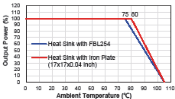
VCQ75U-36xxS (-D) Derating Curve with Heatsink Iron Plate (Vin=36V)
