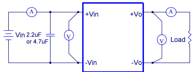
Figure5 EC1TAN Series Single output Test Setup
