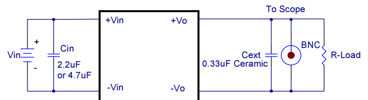
Figure6 Output Voltage Ripple and Noise Measurement Set-up
