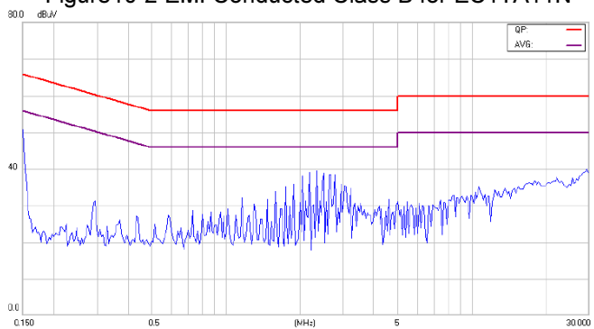
Figure11-2 EMI Conducted Class B for EC1TA21N
