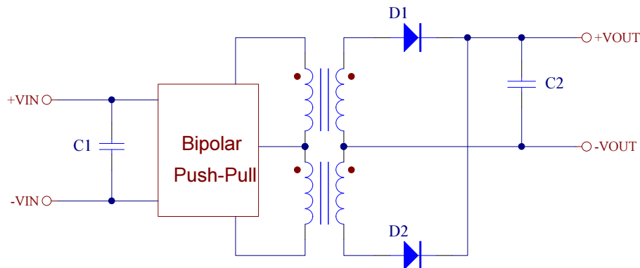
Figure1 Electrical Block Diagram
