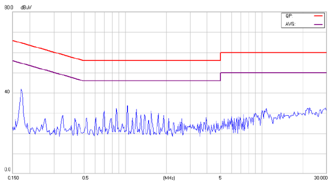
Figure10-2 EMI Conducted Class B for EC1TA11N
