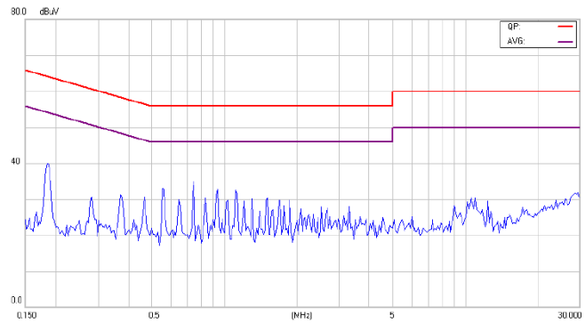
Figure9-2 EMI Conducted Class B for EC1TA01N
