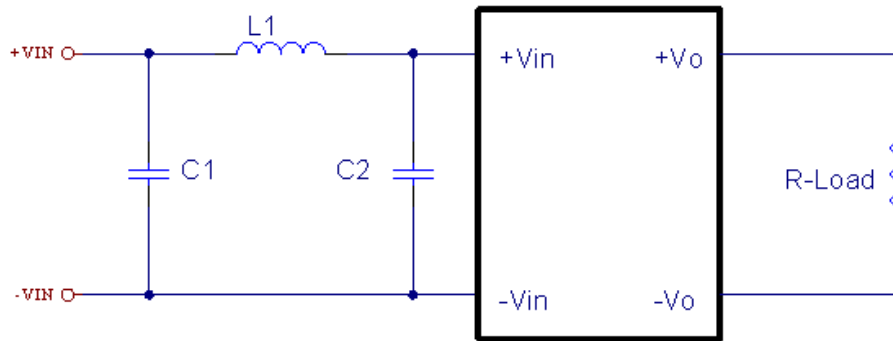
Figure8 Connection circuit for conducted EMI testing
