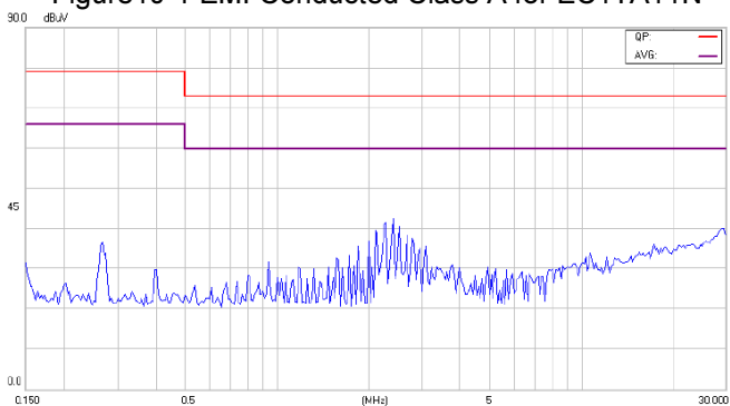
Figure11-1 EMI Conducted Class A for EC1TA21N
