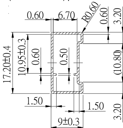
Figure13 SIL Packages Tube for EC1TA0XN and EC1TA1xN
