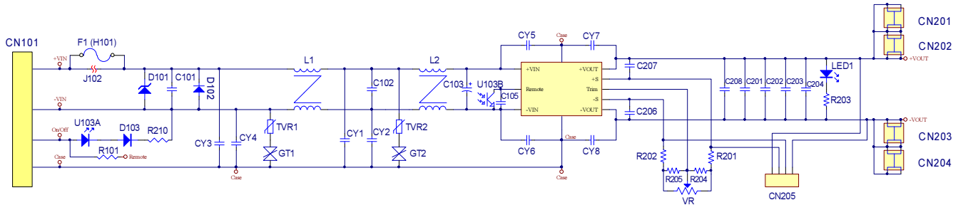
Figure1 Schematic
