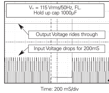
XIII-a. Input Line Dropout
