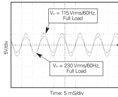
IX-a. Harmonic Distortion
