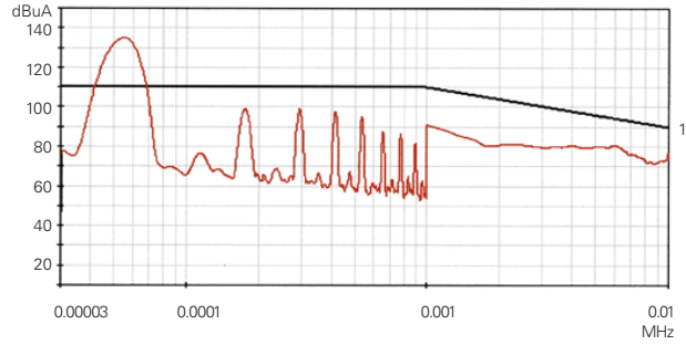
CE101: 120 Vrms, 60Hz, 500W - Without PFF500
