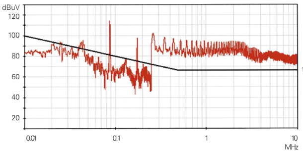
120 Vrms, 60Hz, 500W - Without PFF500
