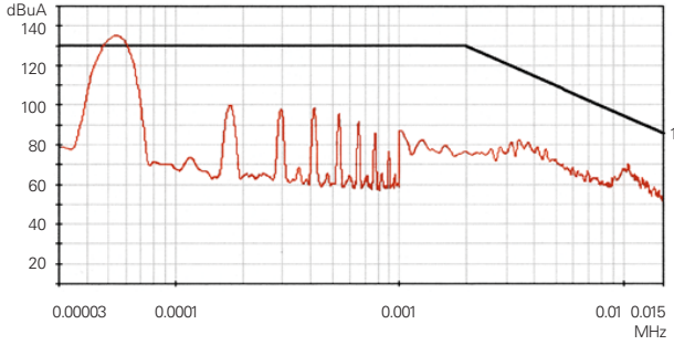
CE01: 120 Vrms, 60Hz, 500W - Without PFF500
