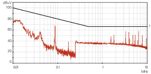
120 Vrms, 60Hz, 500W - With PFF500
