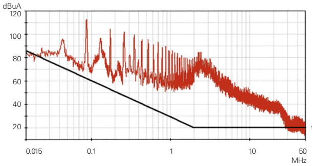
120 Vrms, 60Hz, 500W - Without PFF500
