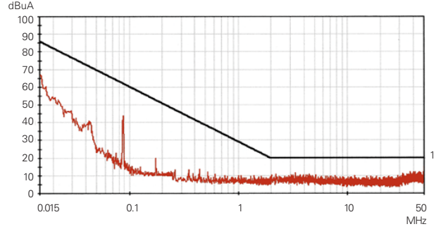
120 Vrms, 60Hz, 500W - With PFF500
