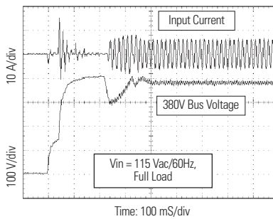
11. Inrush Current vs. Intermediate Bus
