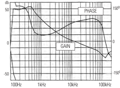
20. Output Converter Voltage Loop Gain & Phase (5Vout)
