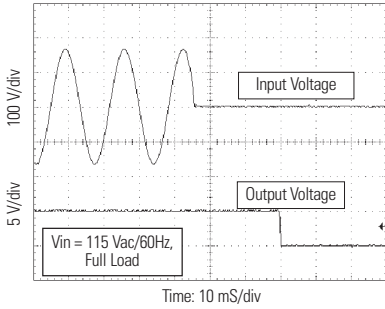
16. Input Voltage Turn-Off vs. Output Voltage
