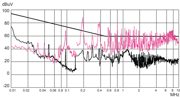
28V in - 150 watts MIL-STD-461D, CE102
