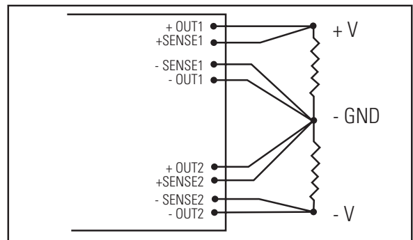
Figure 5: Dual Output (+/-) Operation
