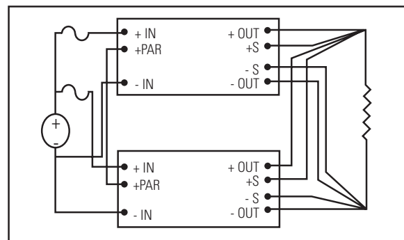
Figure 1c: Parallel Operation
