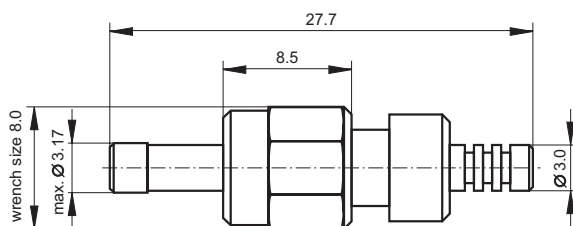
Pic. 4 F-SMA connector with hexagonal nut
