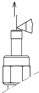
Pic. 10 Cleaving of protruding fiber
