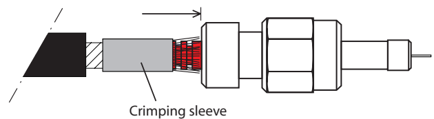
Pic. 8 F-SMA connector with crimping sleeve and boot
