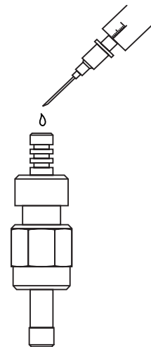
Pic. 7 Filling the F-SMA connector with epoxy
