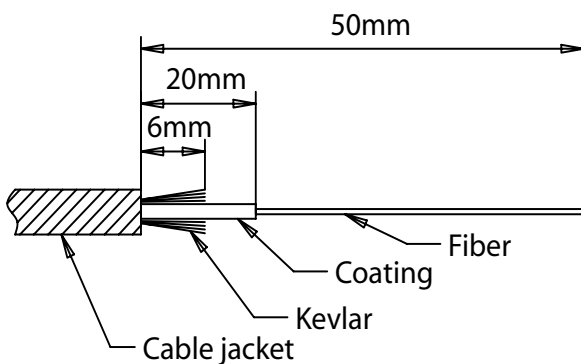
Pic. 6 Stripping dimensions
