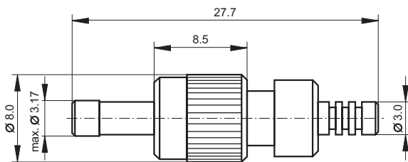
Pic. 3 F-SMA connector with knurled nut
