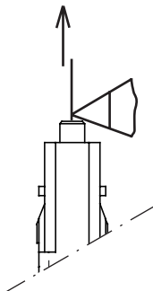
Pic. 8 Cleaving of protruding fiber
