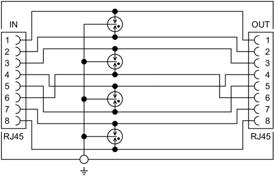
Internal diagram
