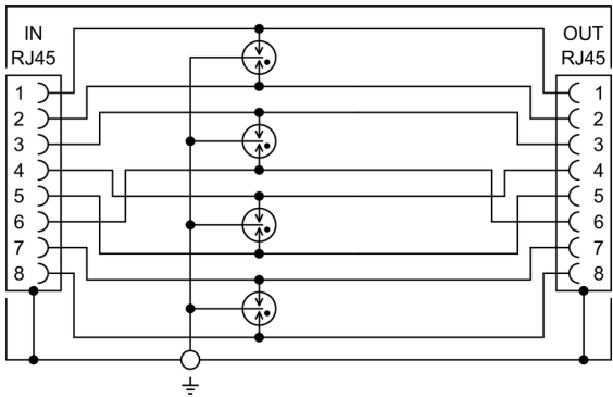
Internal diagram
